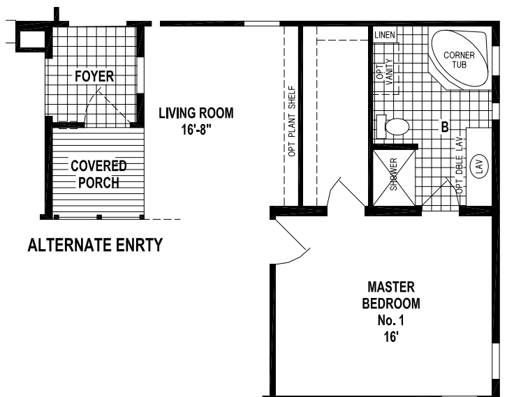
OPTION MASTER SUITE
